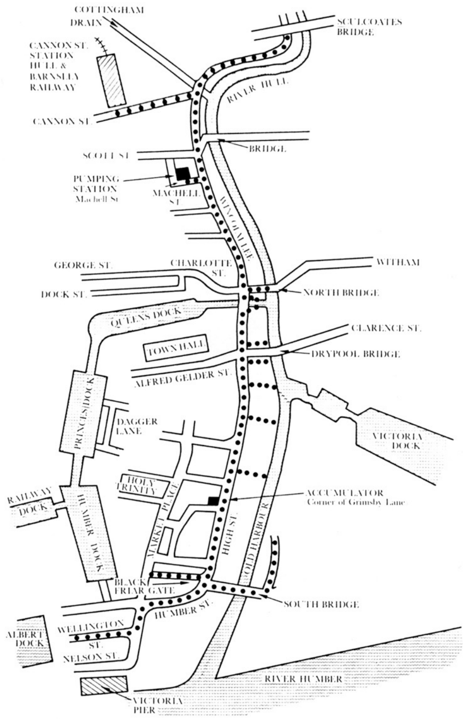
Fig. 4.2 MAP OF HULL HYDRAULIC POWER CO. MAINS
